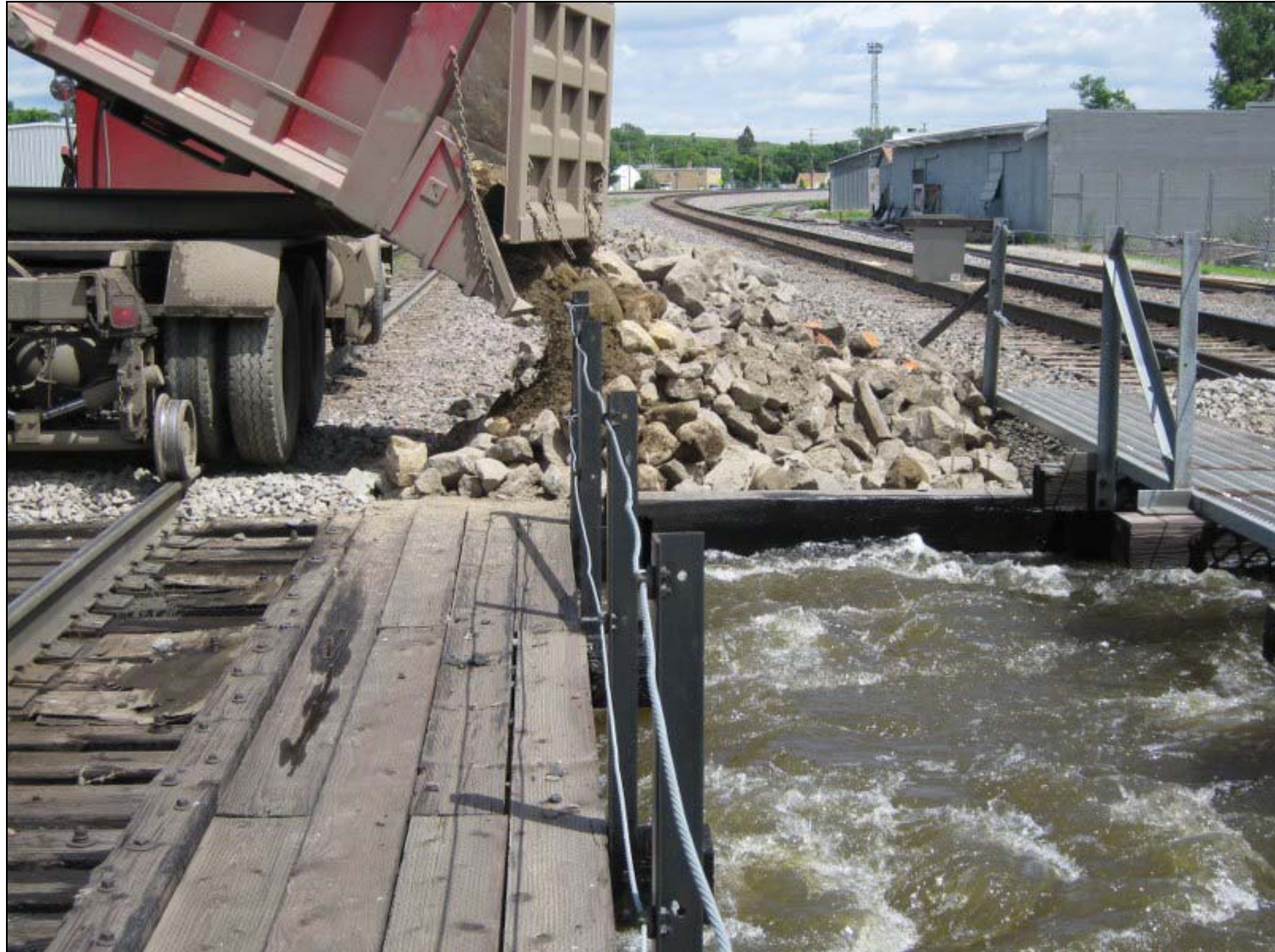
Side-dump truck dumping rip-rap to stabilize soft trackage on mainline bridges crossing Souris River. (Downtown Minot)
